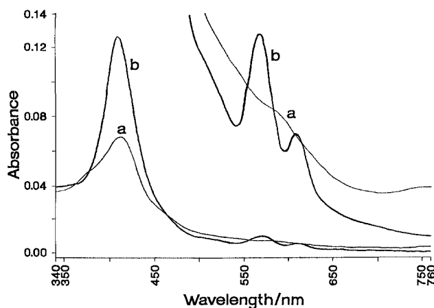
Fig. 1 Spectra of a [(\text{FeTPP})_2\text{O}]^+\text{SbF}_6^- in dichloromethane at 298 K, b "a" after reaction with excess of QBr. Main spectrum: absorbance from 0 to 1.4. Insert spectrum: absorbance from 0 to 0.14.
